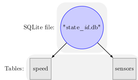
Figure 3. Vehicular database structure (SQLite)
